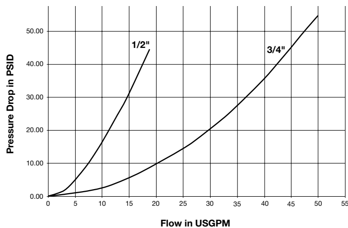
59 Series (1/2" & 3/4") Test Fluid: Oil - 150 SUS
