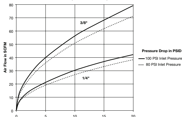
E-z-mate Series (1/4" & 3/8" sizes)
