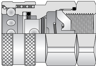
Cylindrical Pneumatic Valve
