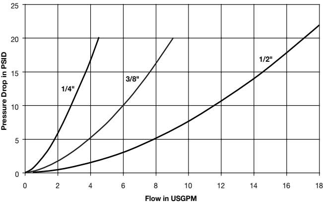
FF Series (1/4", 3/8", 1/2") Test Fluid: Oil - 200 SUS
