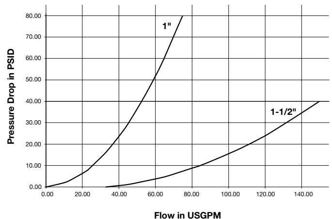
59 Series (1" & 1-1/2") Test Fluid: Oil - 150 SUS
